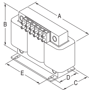
IP00 (Open) – 45 Amps (fundamental) and Below
