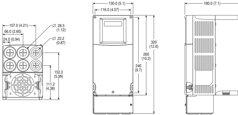
Frame C (Shown with IP30, NEMA/UL Type 1 conversion kit.)
